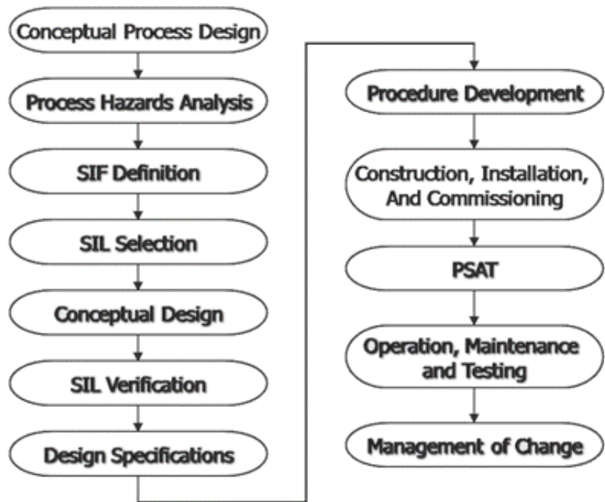
Figure 3 – Kenexis Safety Lifecycle
